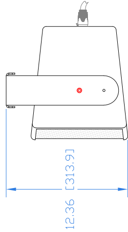
MOUNTING POSITION 2
