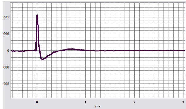
Figure 3.2.4: Impulse Response Displaying Response of Same Horn, with Preconditioning Filter Applied
