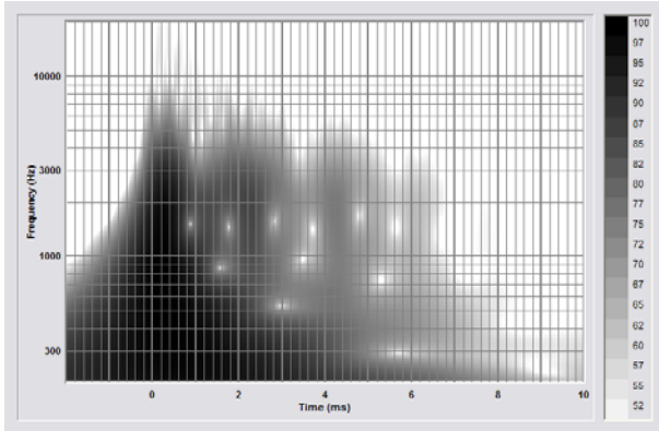
Figure 3.3.3: Cone Speaker, 0.38 m, 15 degrees Off Axis, No Filtering
