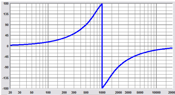
Figure 3.4.4: Ideal Correction Filter (blue) - Phase Response
