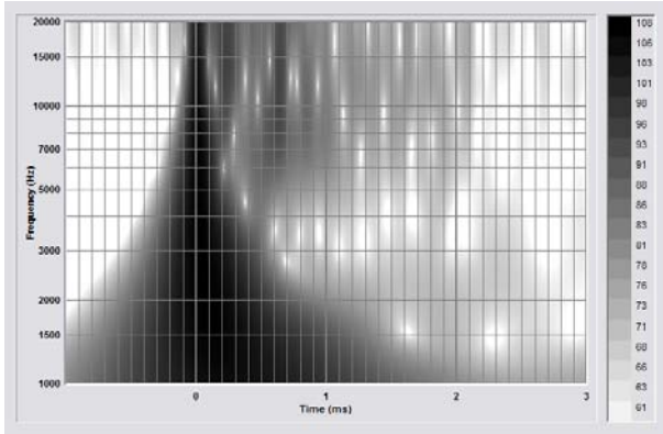
Figure 3.1.2: Spectrogram Displaying Phase Plug Transient Smear - Axial Response, 50 dB Scale
