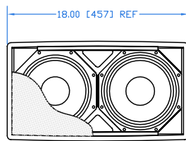
GRILLE PARTIALLY SHOWN
