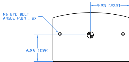
GRILLE PARTIALLY SHOWN
